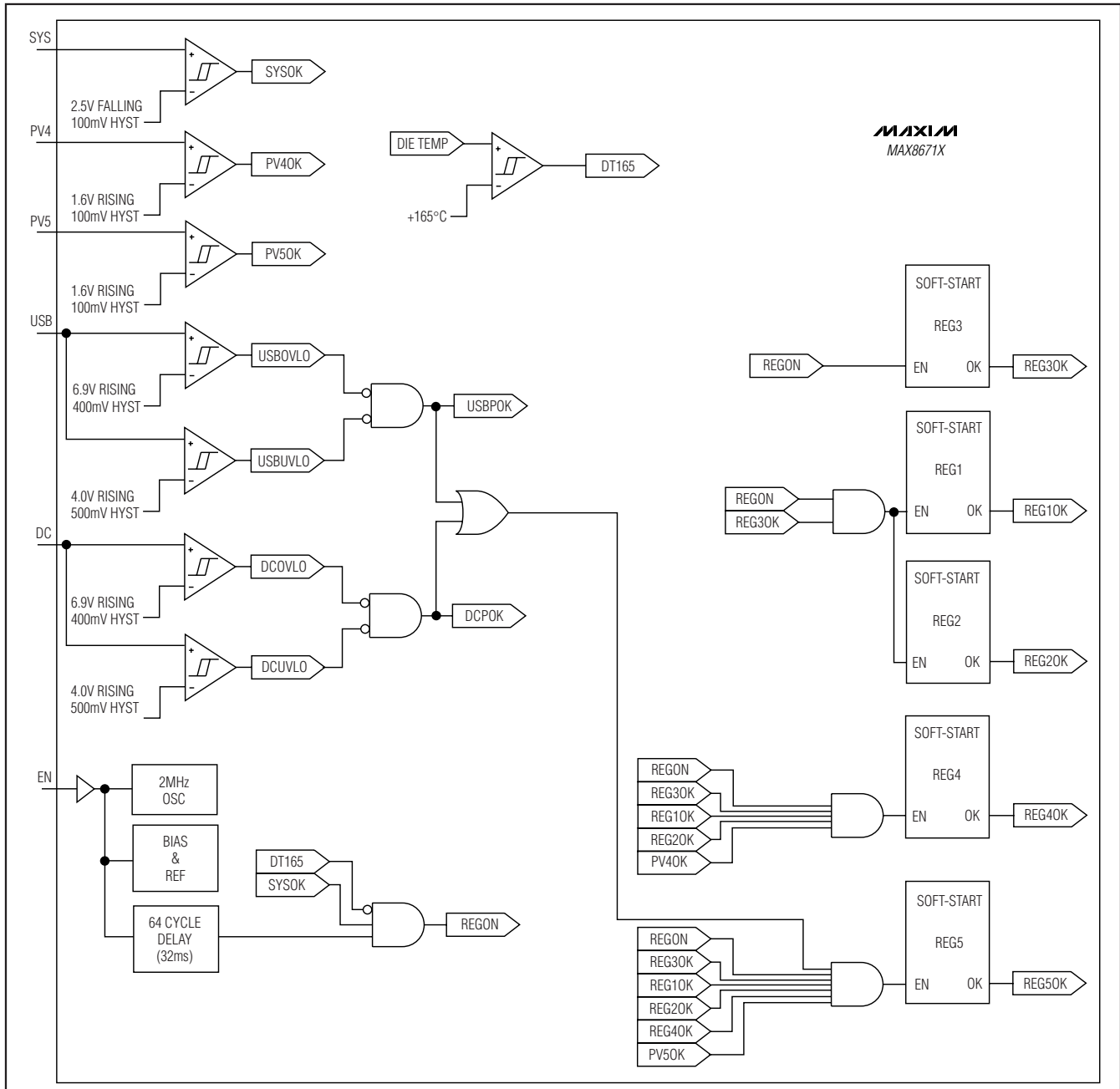
Figure 11. Enable/Disable Logic
